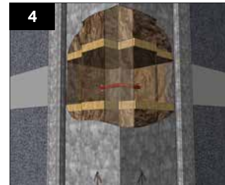
Cutaway section of corner showing void for cable to run through corner to the adjacent wall. Note earth-wool will be within the void, but this can easily be pushed out of the way.
