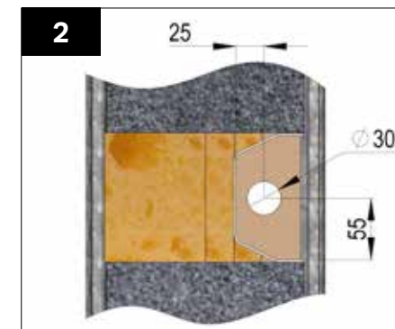
Position hole approximately central to the cable management channel and around 30mm in diameter but no larger than 38mm.
