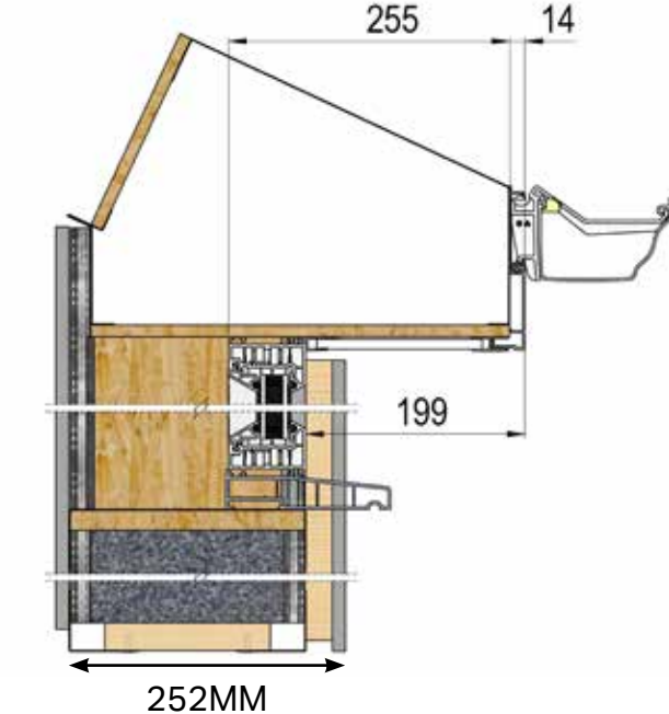
HUP! WITH 199MM SOFFIT FROM EXTERNAL FRAME
