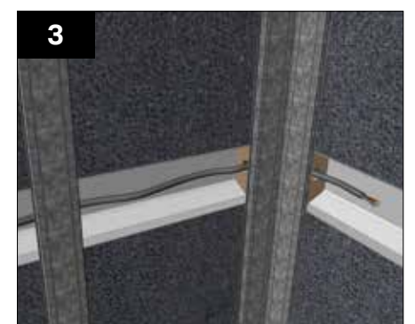
Run cable through the drilled holes. If cable needs to run vertically up the wall from the cable management channel, run this cable in conduit.
